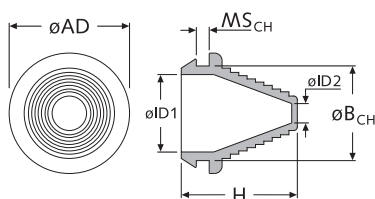
Membrane grommets with variable inner diameter
