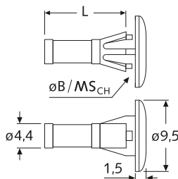
Flachkopf-Stützpfeiler PCB support pillars with flat head
