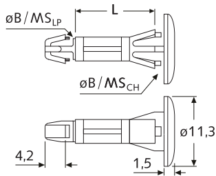
Flachkopf-Distanzhalter Flat-head PCB spacers
